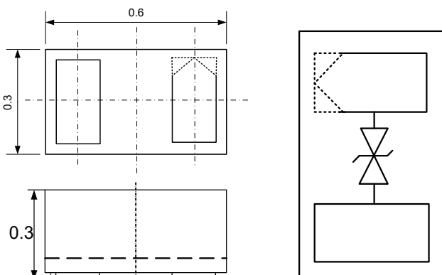
Package Dimensions
